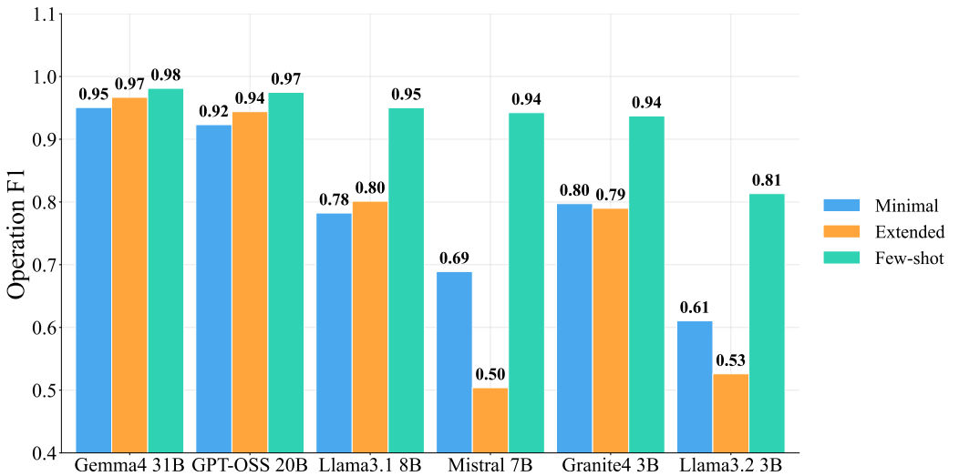
Figure 1. Operation-level F1 by model and prompting regime. Few-shot prompting (teal) yields the best accuracy for all six models and sharply compresses the gap between small and large models; the extended prompt (orange) is inconsistent, degrading Mistral 7B and the Llama3.2 3B small model relative to the minimal prompt (blue).
